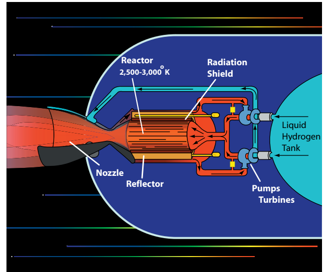
Proposed nuclear thermal rocket engine
